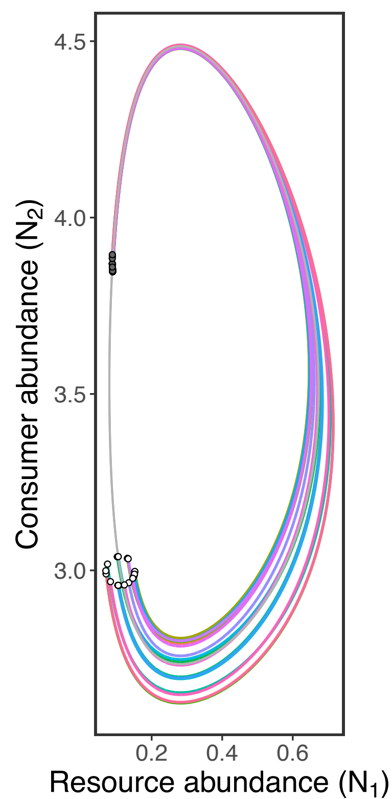
(a) 2-species equilibrium point with periodic forcing
