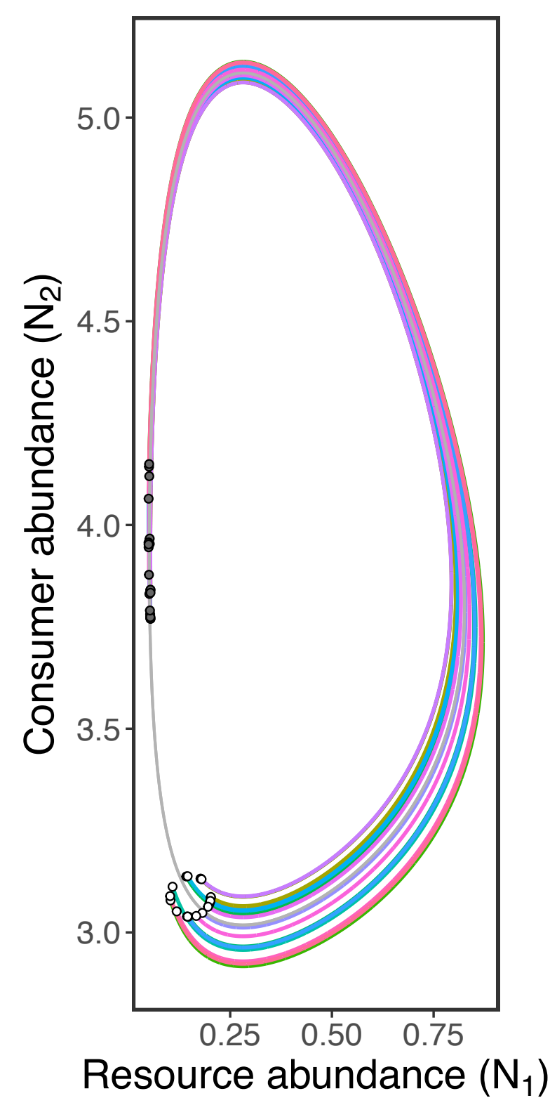
(b) 2-species limit cycle
