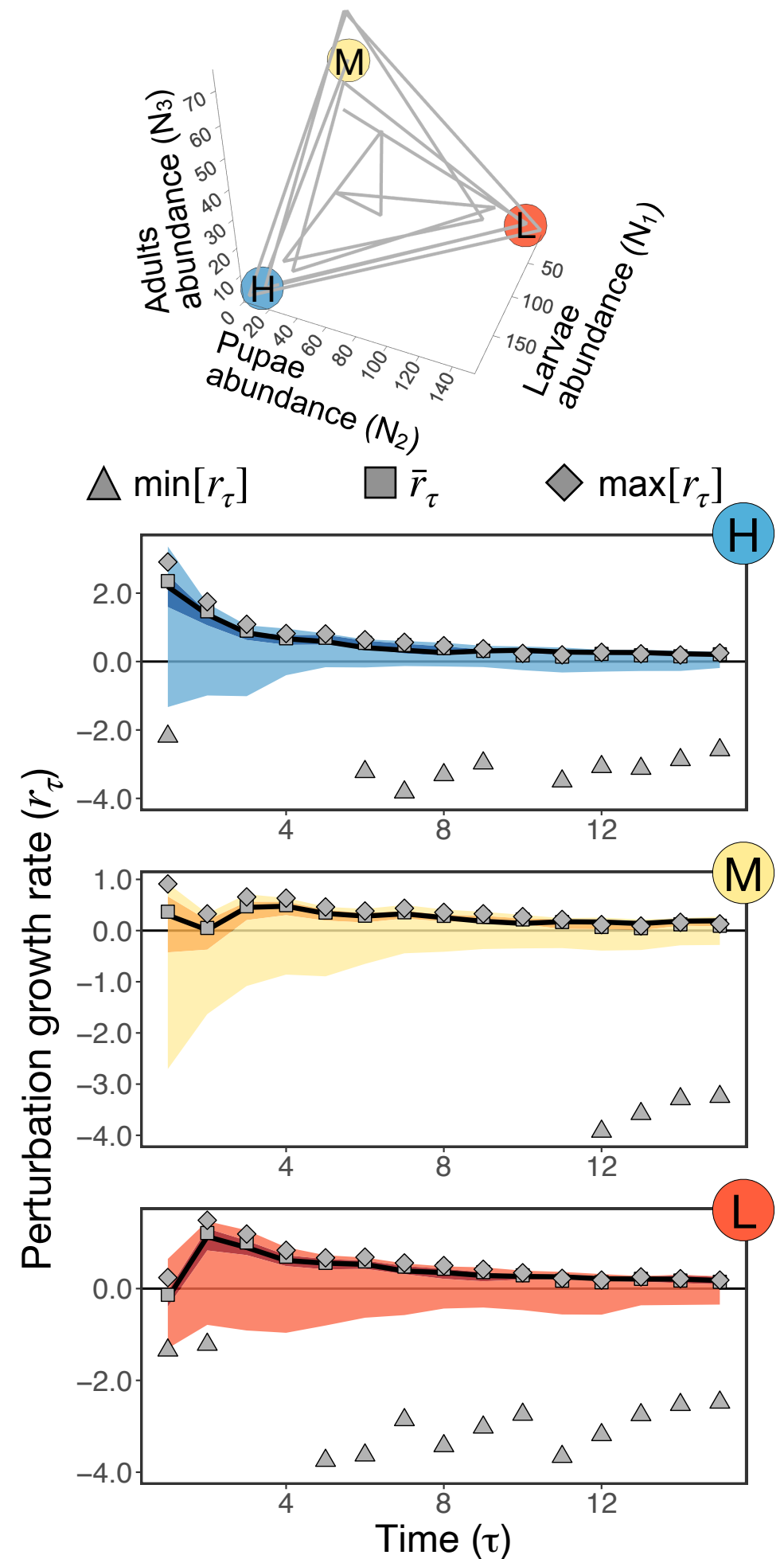
(b) 3-stages discrete-time chaotic attractor
