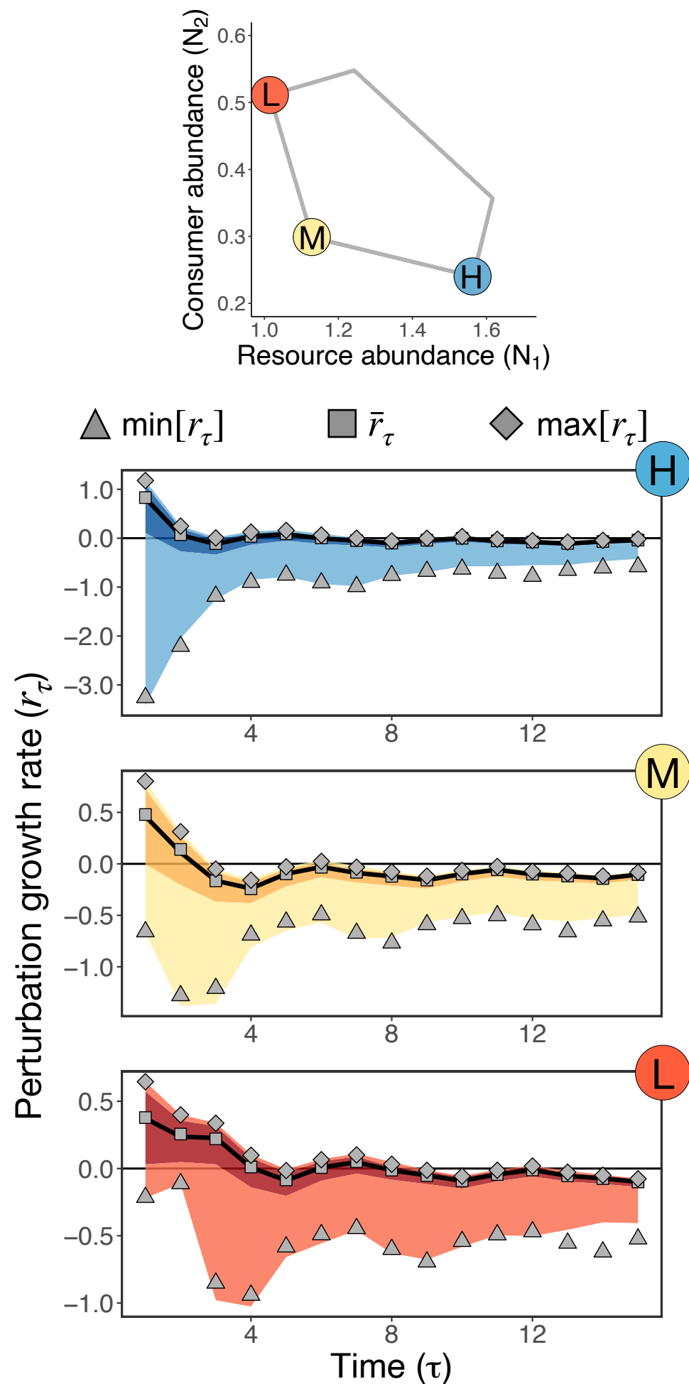
(a) 2-species discrete-time limit cycle
