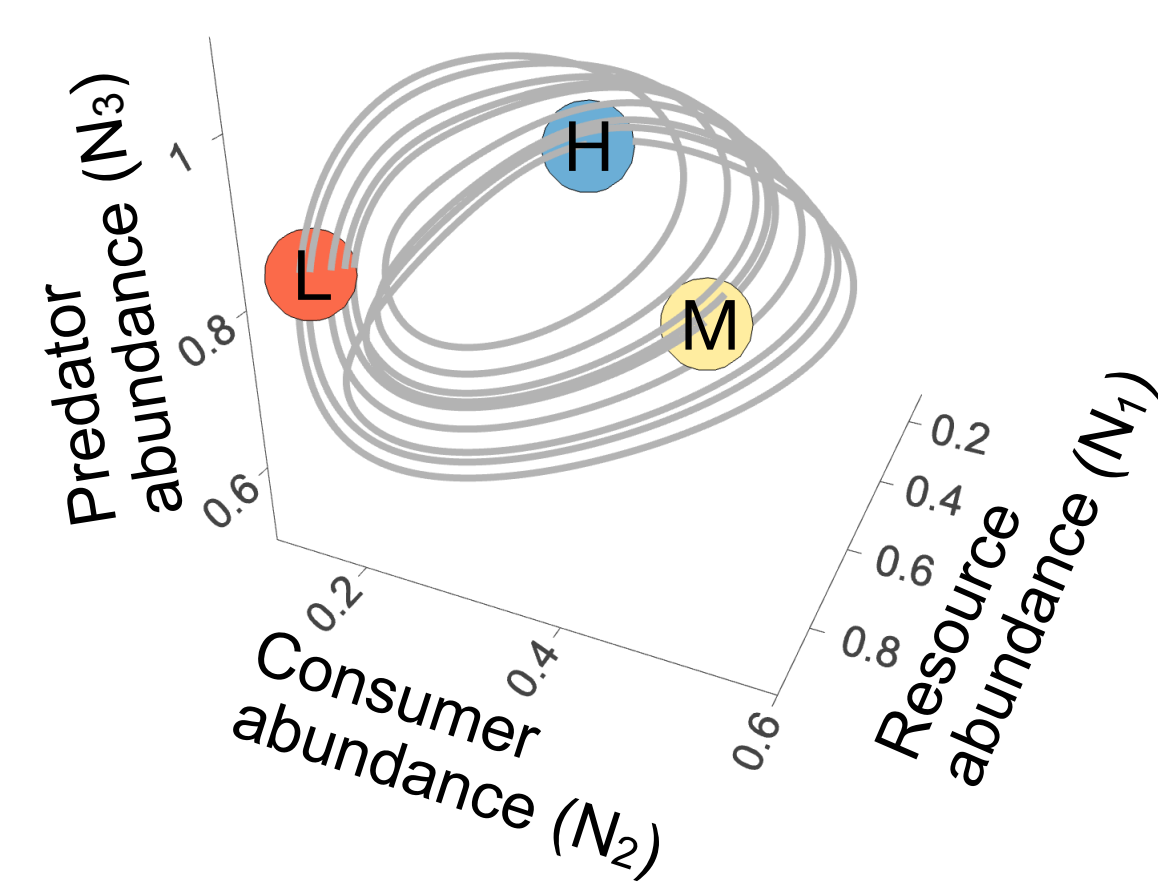
3-species chaotic attractor
