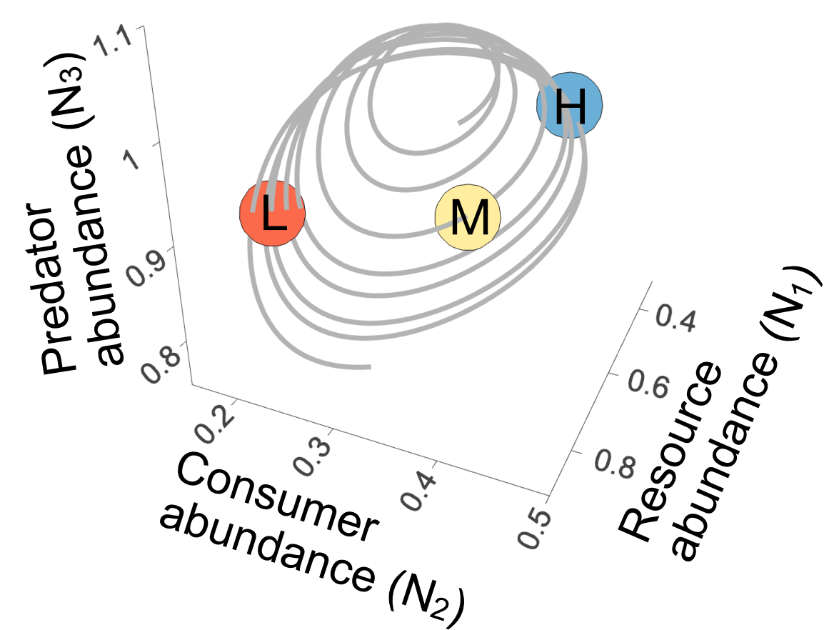
3-species limit cycle with nonstationary forcing
