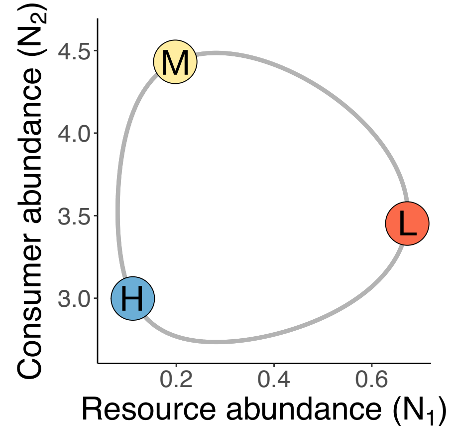
2-species equilibrium point with periodic forcing
