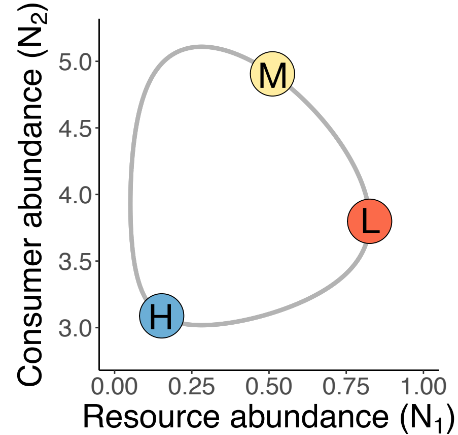
2-species limit cycle
