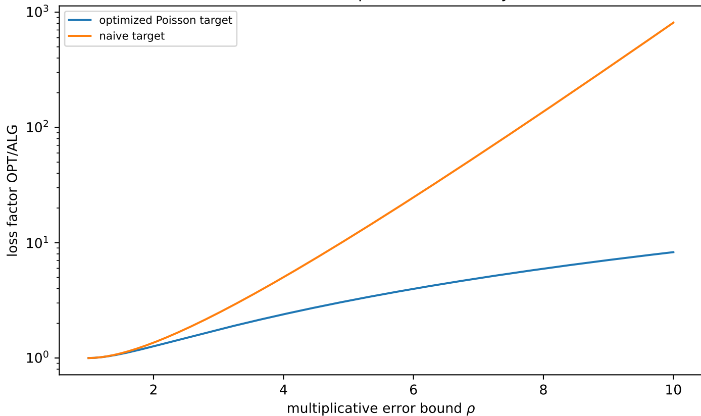
Continuous Poisson predicted-intensity model
