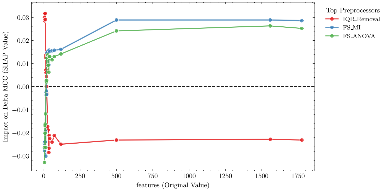
Top 3 Preprocessors Impact vs features
