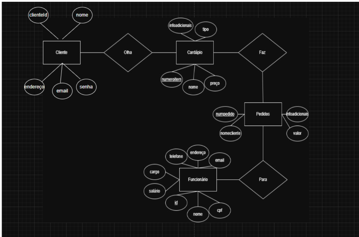
Diagrama E-R
