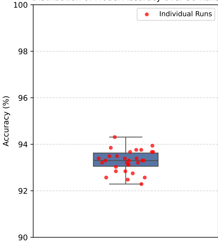
Distribution of Model Accuracy over 30 Runs
