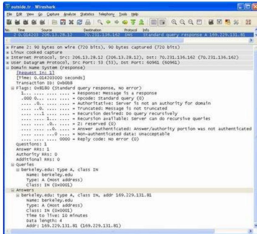
Figure 11-13. A response generated by GW.HOME and destined for the client. This message completes the recursive DNS transaction.
