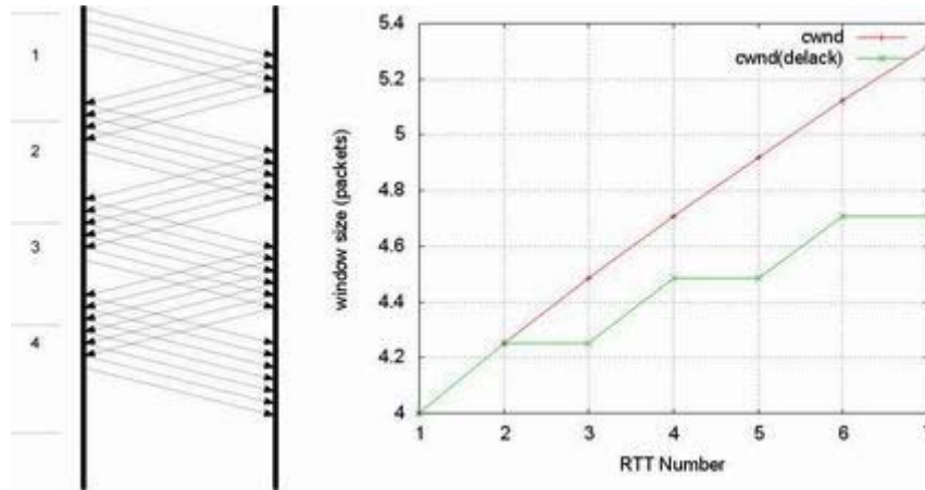
Figure 16-3 (left) illustrates the operation of congestion avoidance. Once again, the numbers are in units of the RTT of the connection. Assuming the connection sends four packets (top), four ACKs are returned, allowing cwnd to grow slightly. By the second RTT period, the growth is enough to overcome the integer rounding and cause an increase of one SMSS to cwnd , allowing one additional packet to be sent. The growth of cwnd as a nearly linear function of time is illustrated on the right, on a linear-linear plot. The second line to the right shows how cwnd grows when every other packet is acknowledged, simulating the use of delayed ACKs. In this case, the growth is still about linear, but not as rapid.
