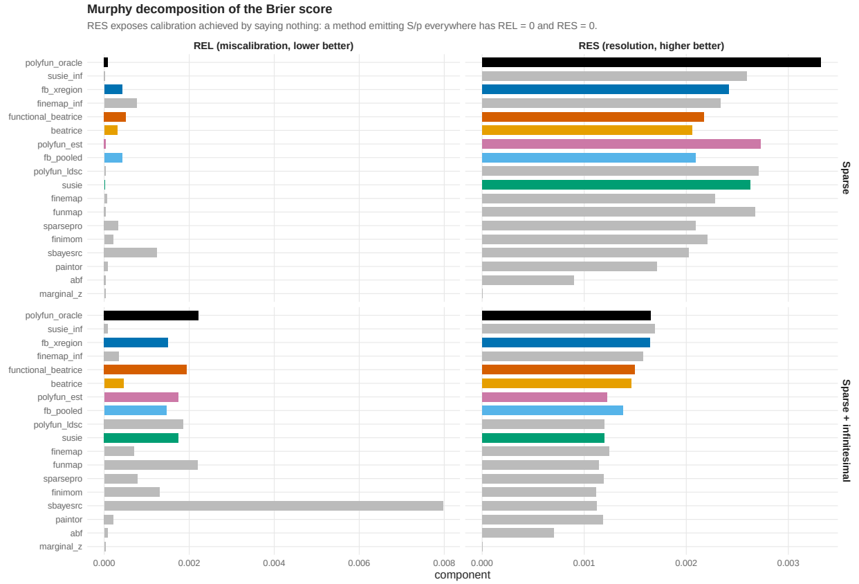
Figure 10: Murphy decomposition. REL is miscalibration (lower better); RES is resolution (higher better). RES is what distinguishes an informative posterior from one calibrated by being vague.
