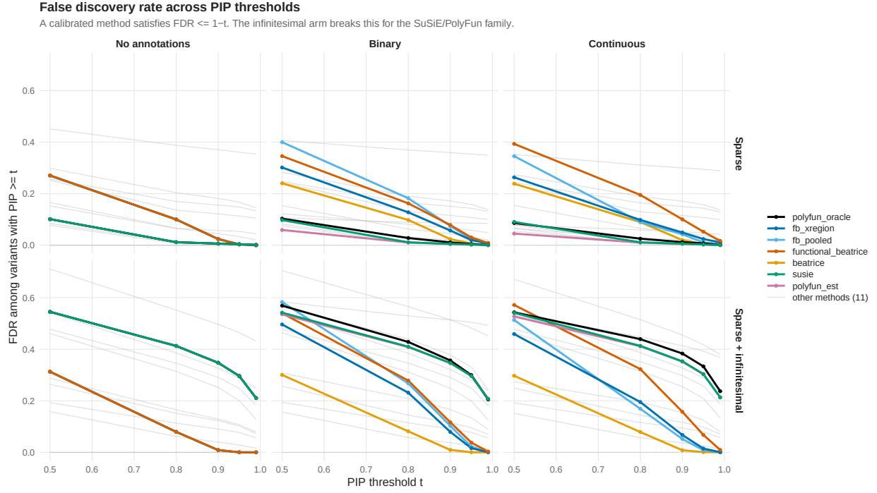
Figure 9: FDR across PIP thresholds. A calibrated method satisfies FDR_t \leq 1 - t .
