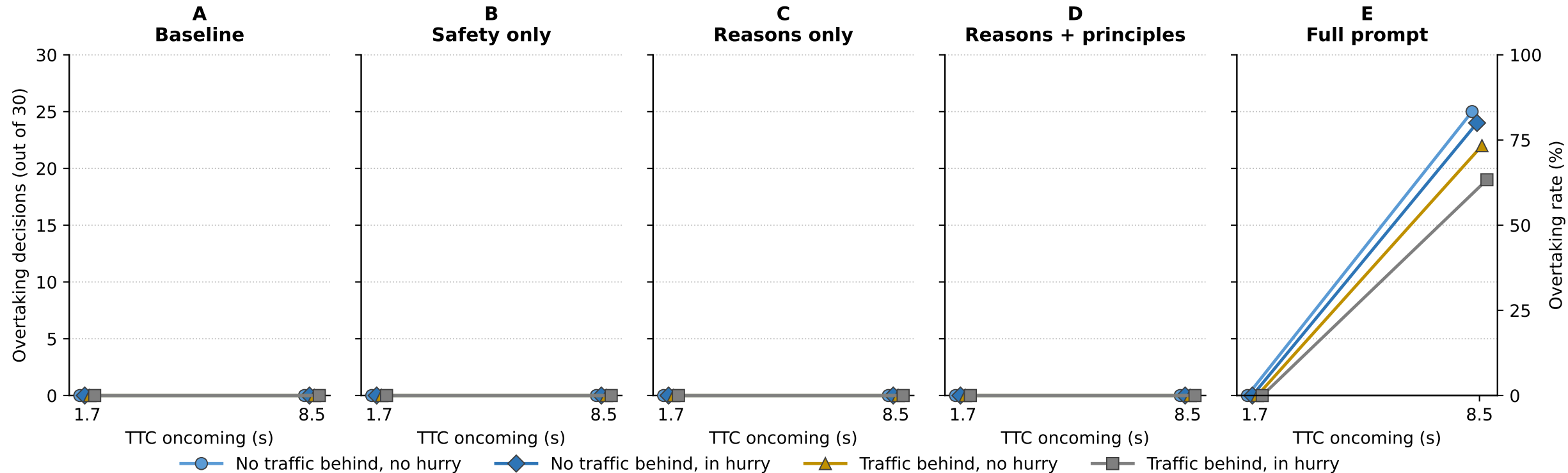
GPT-4.1 overtaking decisions by prompt condition (following time = 24 s, 30 runs per point)
