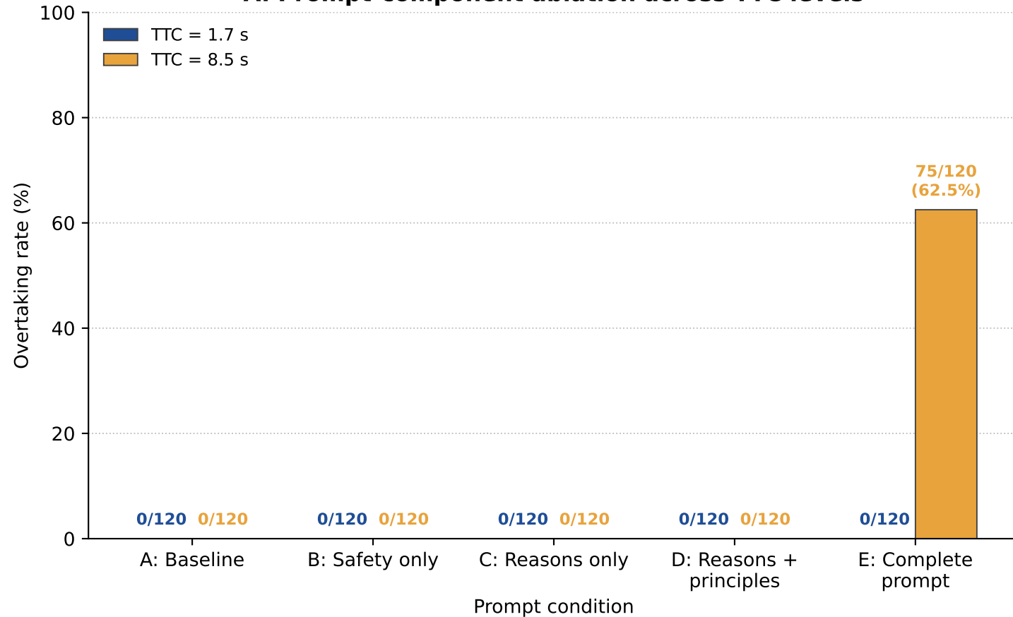
A. Prompt-component ablation across TTC levels
