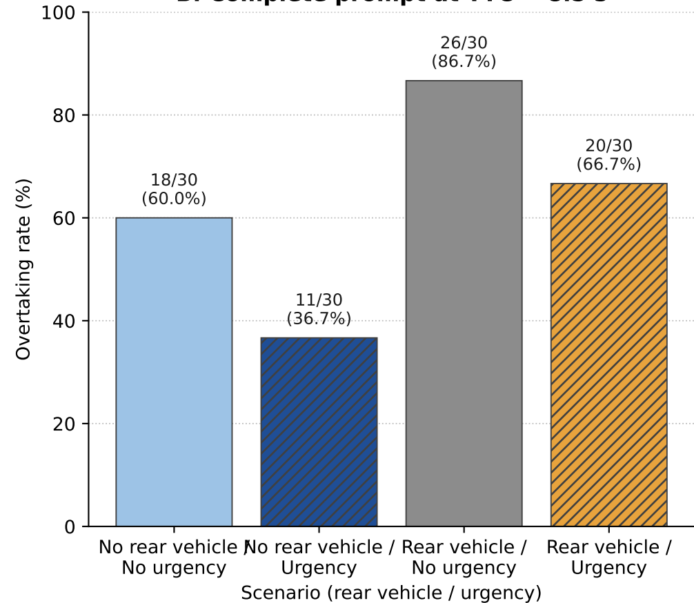
B. Complete prompt at TTC = 8.5 s
