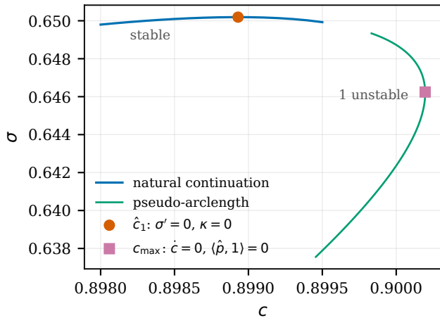
the two kinds of critical point
