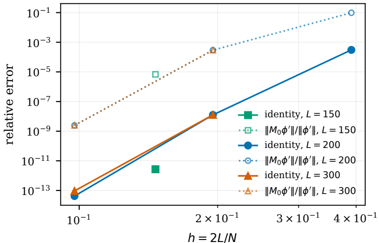
spectral convergence; floor at machine precision
