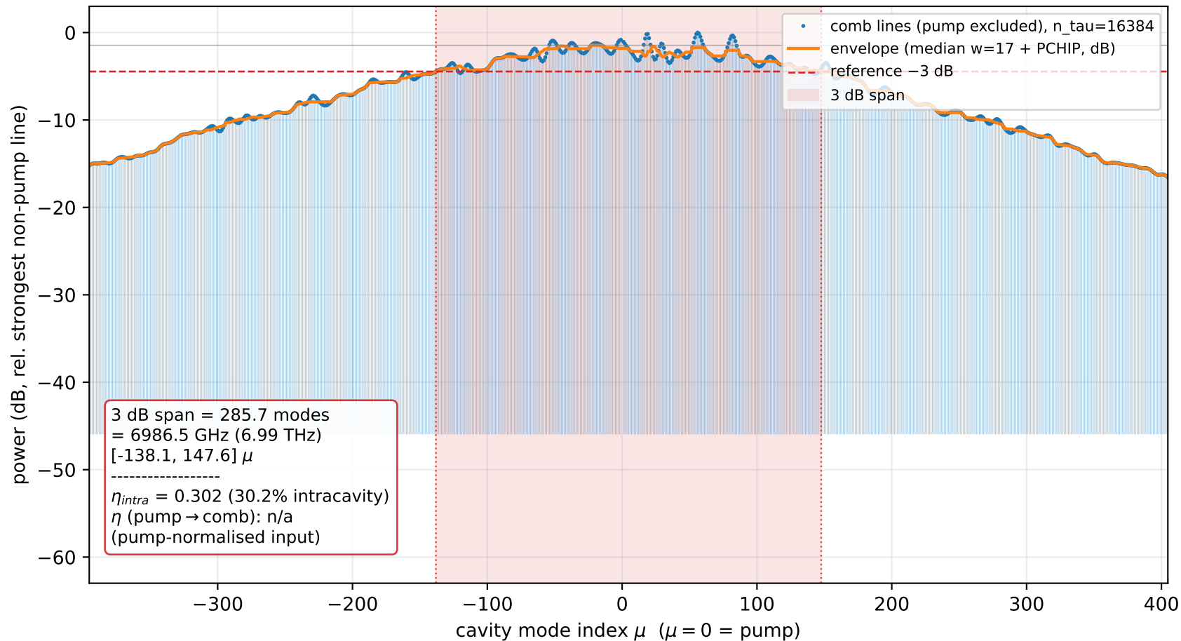
Single-DKS 3 dB spectral span @ \delta\omega = 10.0\kappa (cycle-averaged, None RT)
