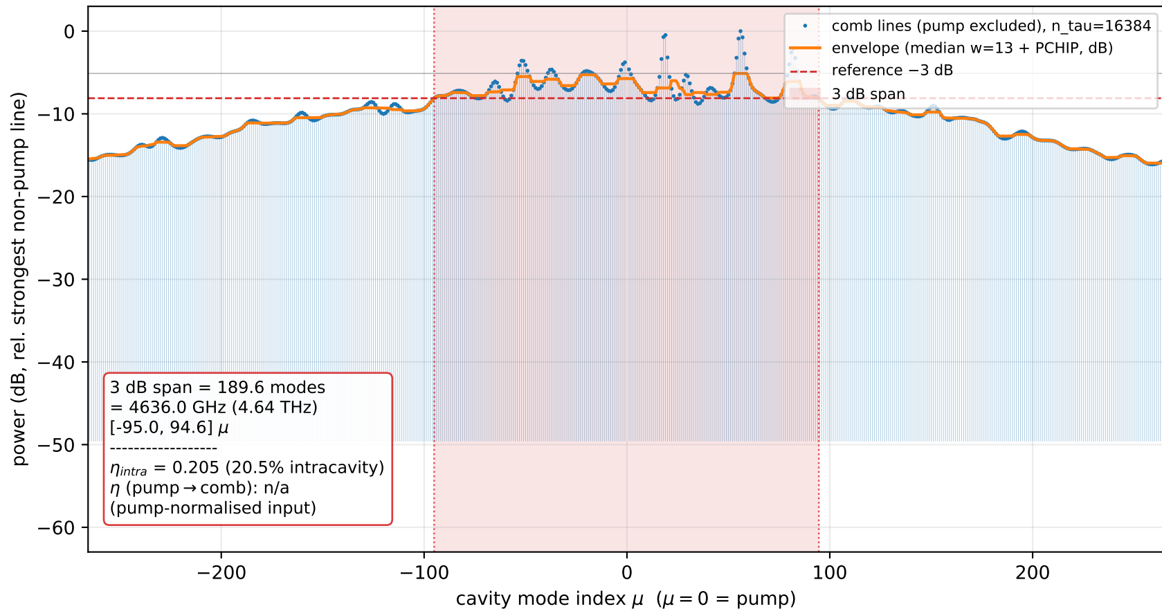
Single-DKS 3 dB spectral span @ \delta\omega = 8.0\kappa (cycle-averaged, 304 RT) breather T~154 RT, dU/U=4.1%
