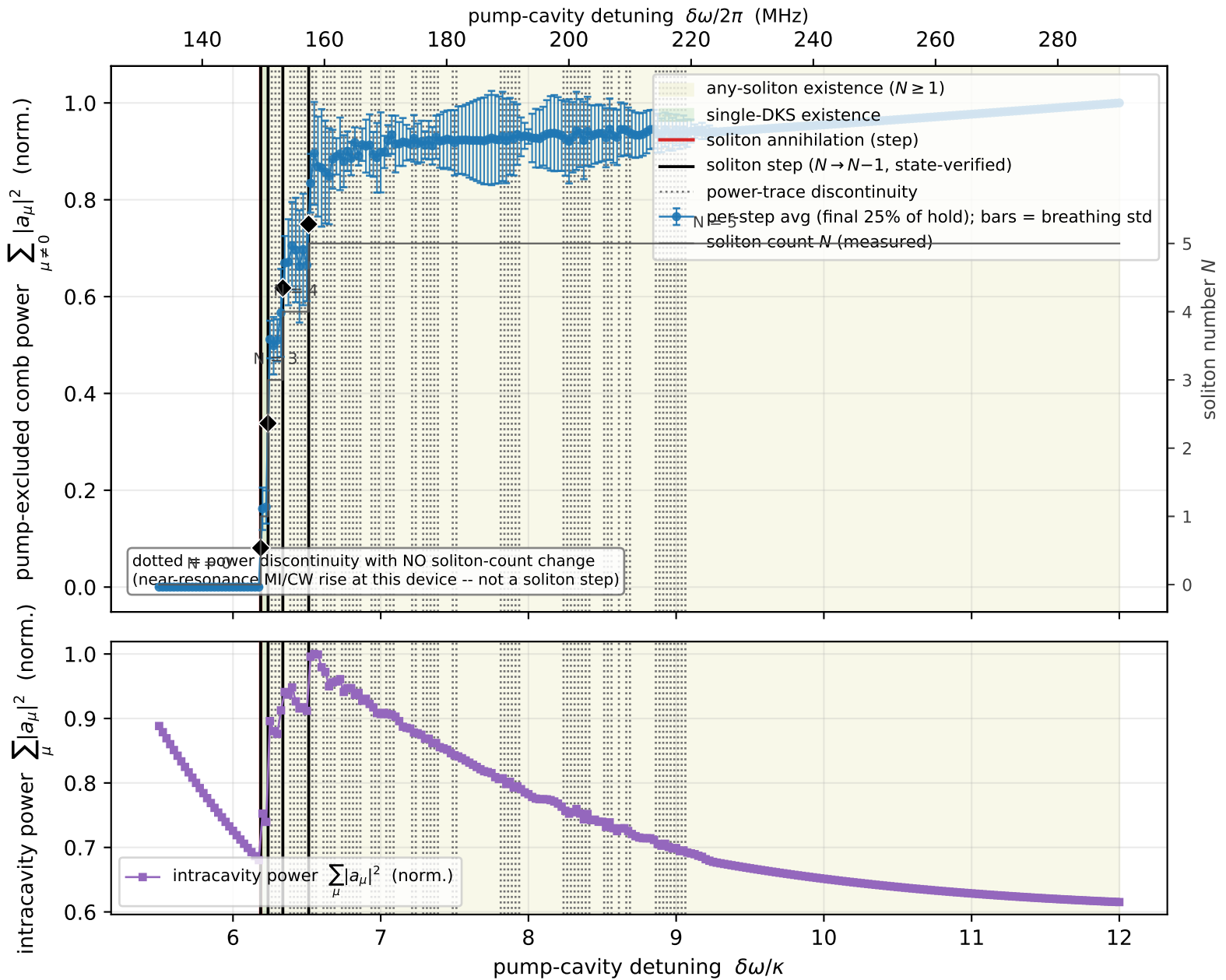
5-soliton staircase, p_{in} = 0.214 W, n_{tau} = 4096 . Deterministic symmetry-broken seed (position_seed=1, jitter=0.25) at 12\kappa , warm continuation swept DOWN, hold 2000 RT/step, averaged over the final 25% (cycle-averages the breather). Thermo-optic model ON (deterministic, noise off). The solitons annihilate sequentially at the branch's lower edge -- the staircase; the final 1 \rightarrow 0 annihilation must never be FORCED to register as a power step (matched only if the untouched detector resolves it naturally on the plotted trace). Green = single-DKS existence region. Olive = any-soliton ( N \geq 1 ) region. Solid black lines mark STATE-VERIFIED soliton steps (power discontinuity coinciding with a measured soliton_count transition); dotted lines mark power discontinuities without a state change. Thin gray staircase = measured soliton count N (twin axis). Raw data, no smoothing.
