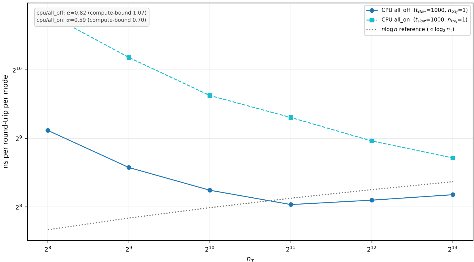
Figure 6 — Solver runtime scaling
