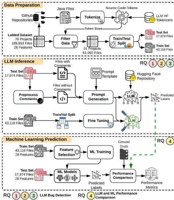
Fig. 3: Main steps of the performed study.
