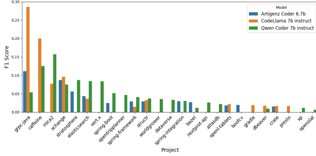
Fig. 4: Zero-shot F1 Score comparison across projects
