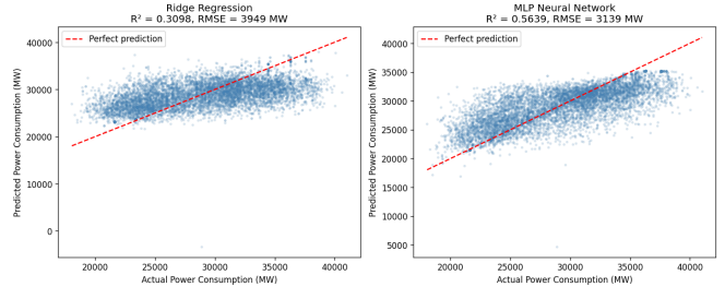
Fig. 4. Predicted vs. actual power consumption on the validation set. Points close to the diagonal indicate accurate predictions.
