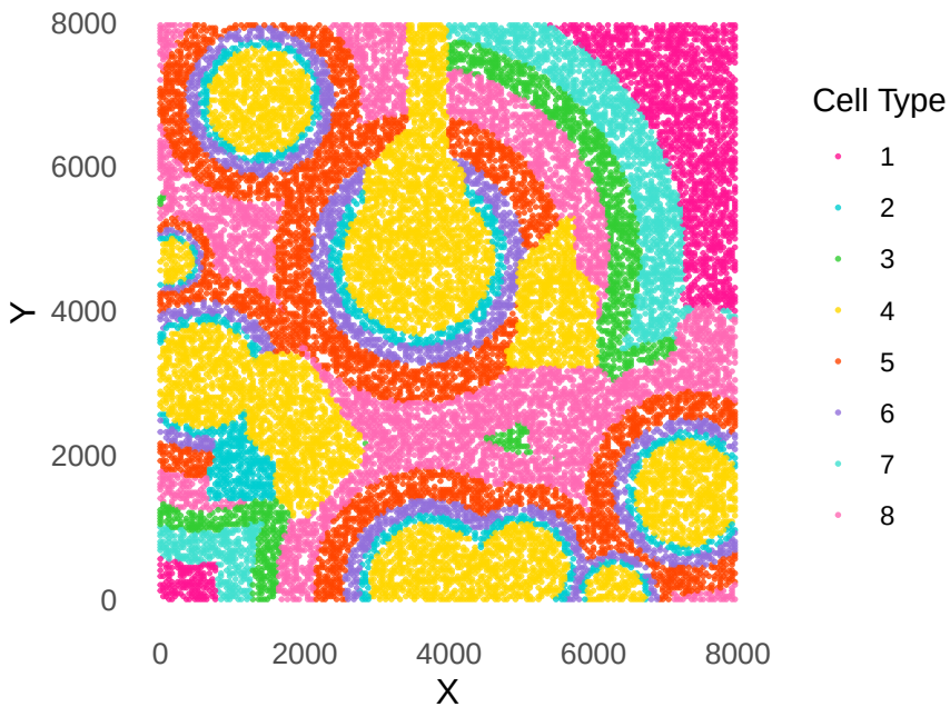
Spatial Transcriptomics Clusters
