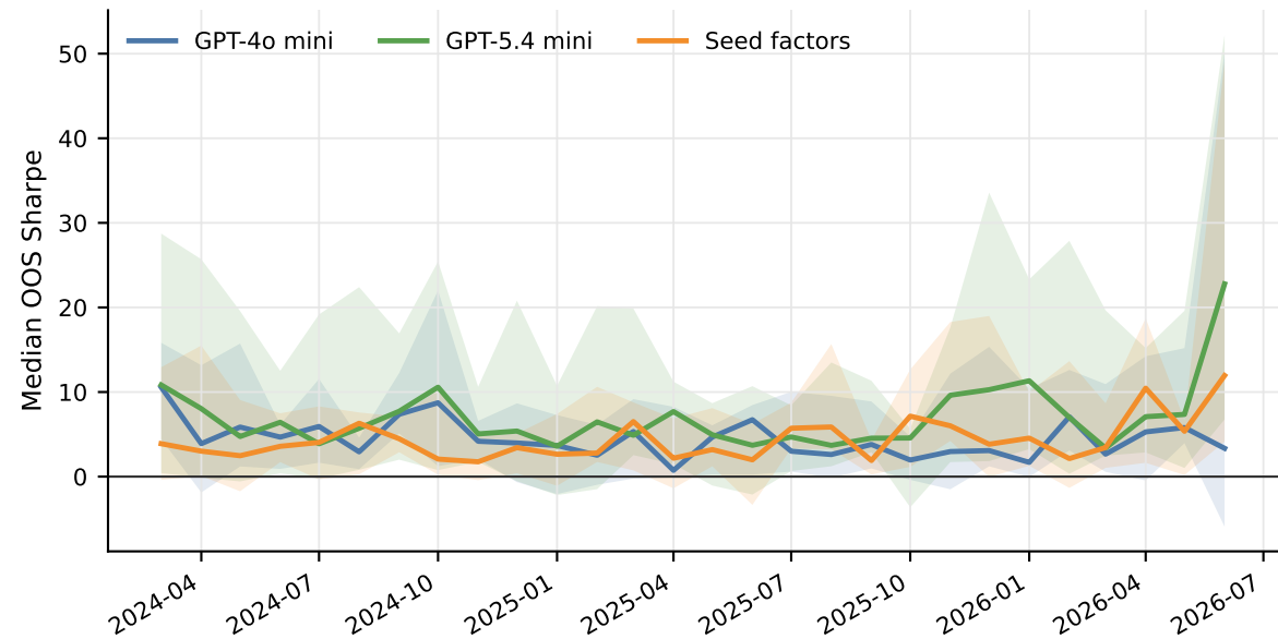
Time stability of ensemble OOS Sharpe
