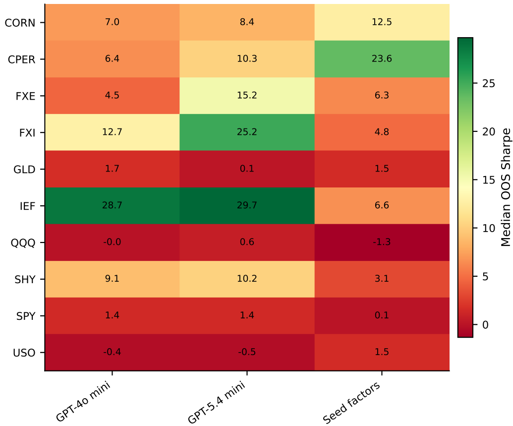
Median ensemble OOS Sharpe by ETF
