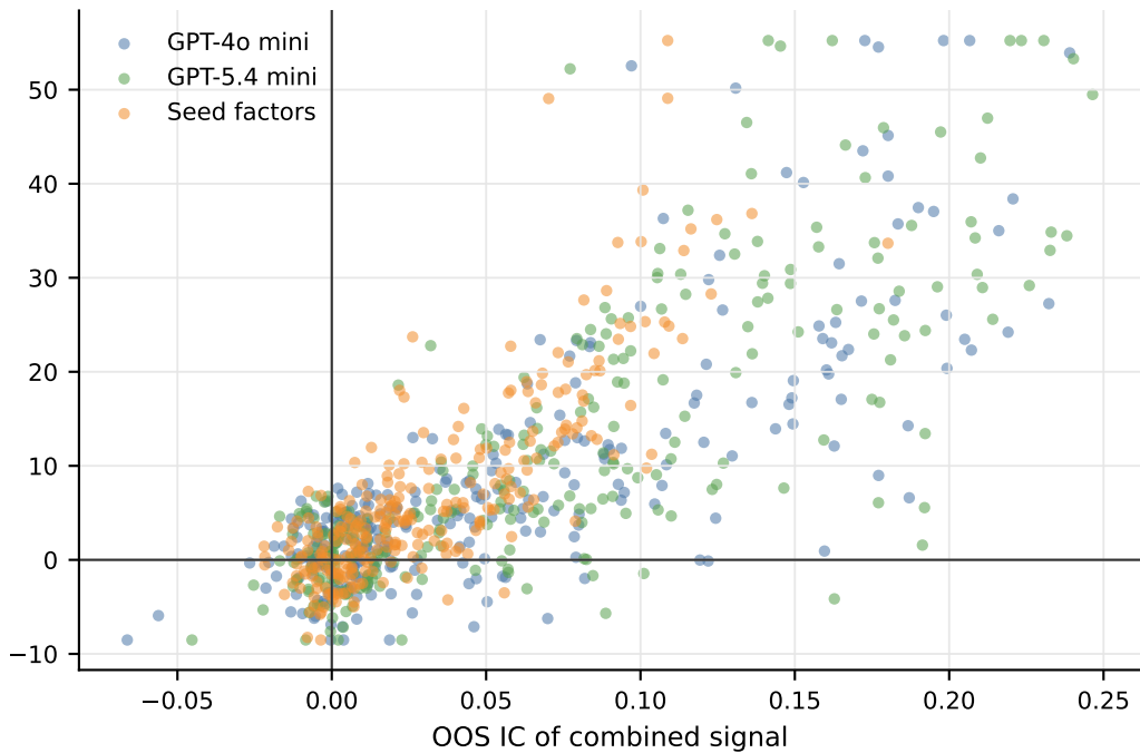
Signal IC versus realised ensemble Sharpe
