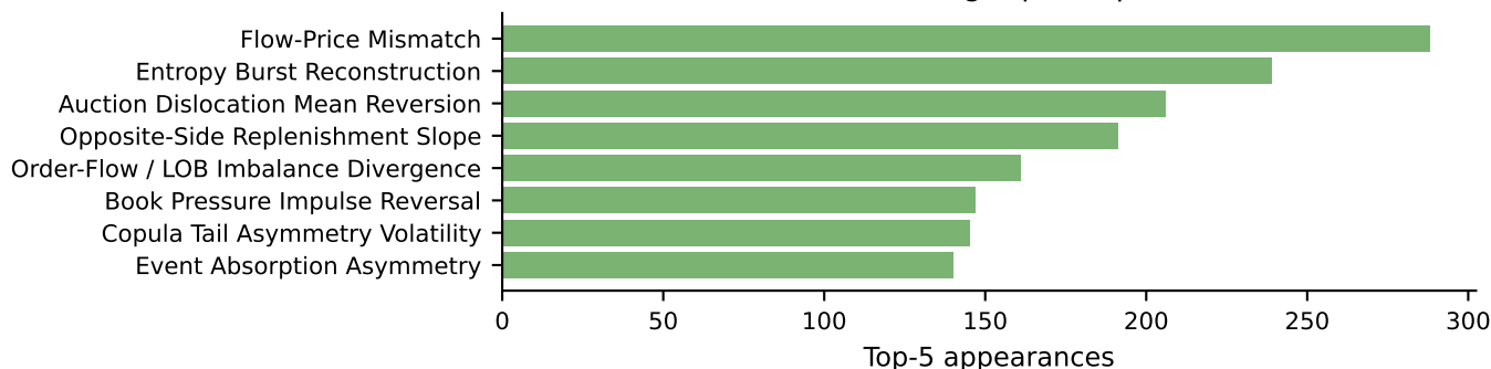
Seed factors: recurring top-5 important factors
