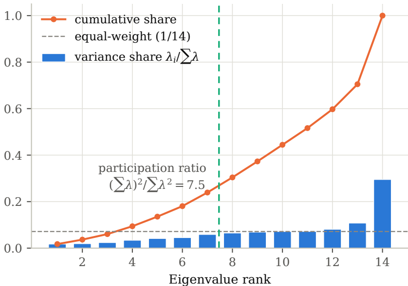
Share of total variance
