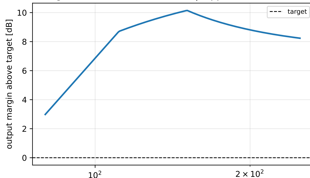
Eighteen Sound 12NTLW3500 | upper-bass channel
