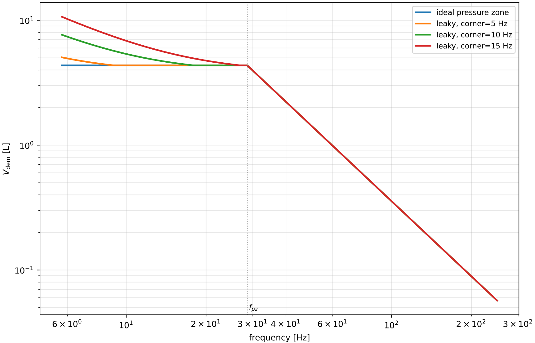
Room-demand sensitivity to leaky corner, 110 dB @ 3 m, 3 m couch basis
