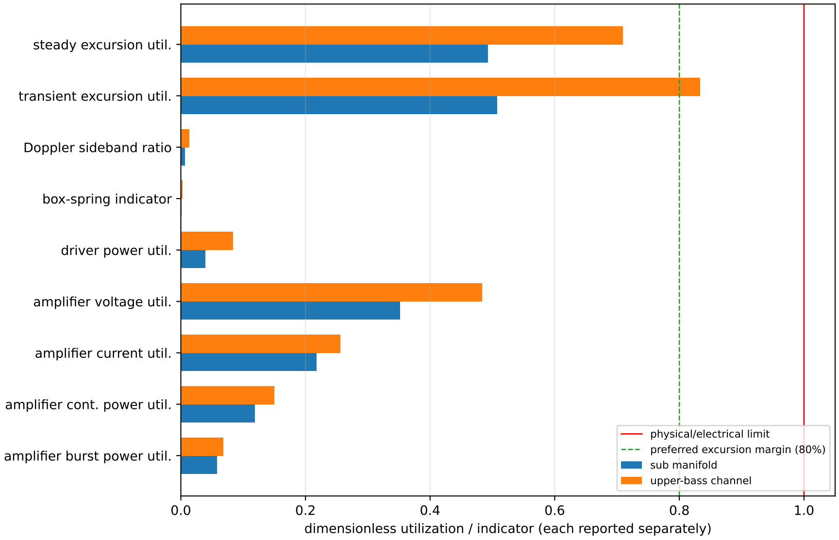
BMS 18N862 (sub) vs. Eighteen Sound 12NTLW3500 (upper) — worked selected pair
