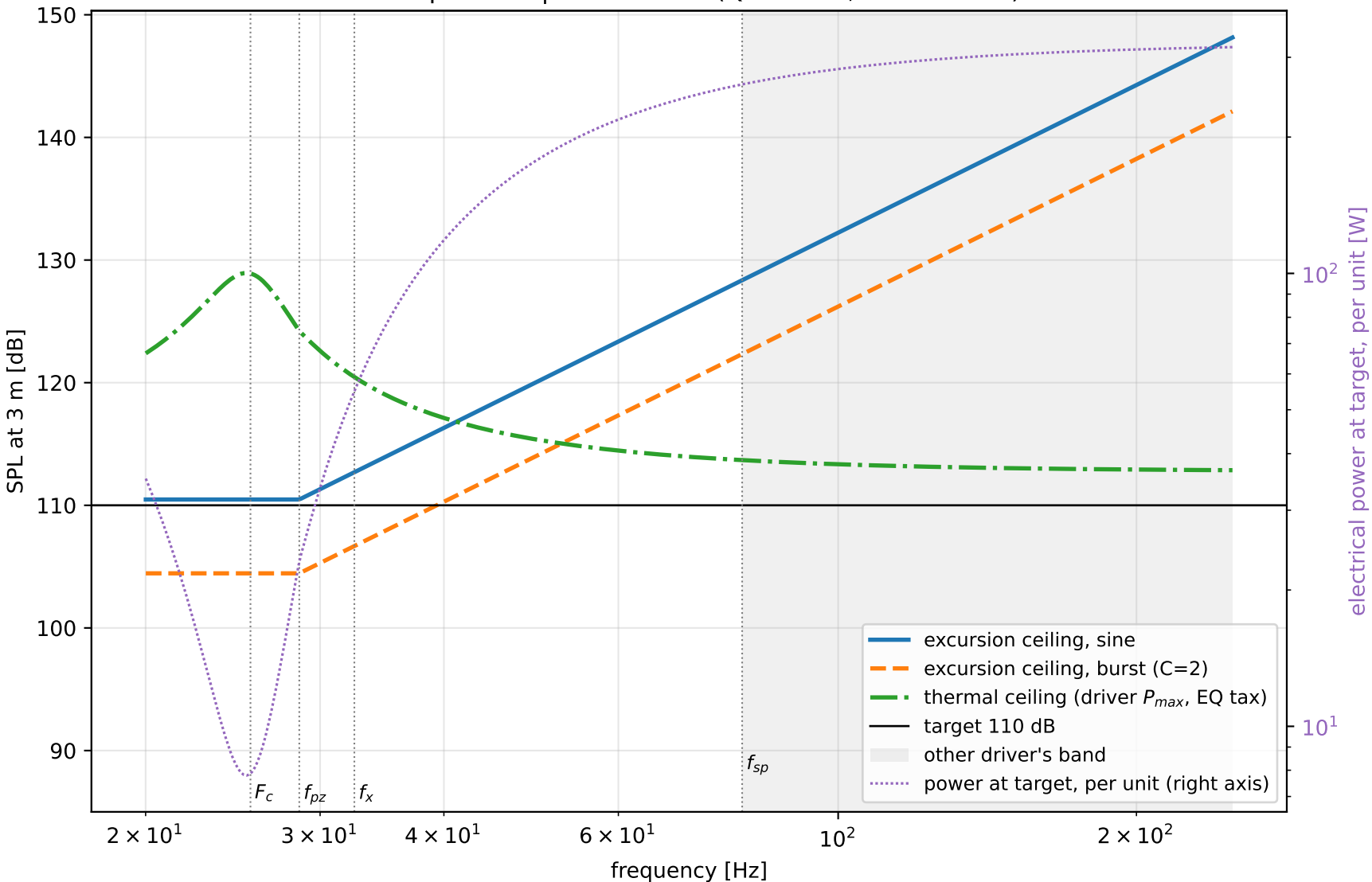
Example S18 | 2x in 473 L (Qtc=0.61, Fc=25.5 Hz)
