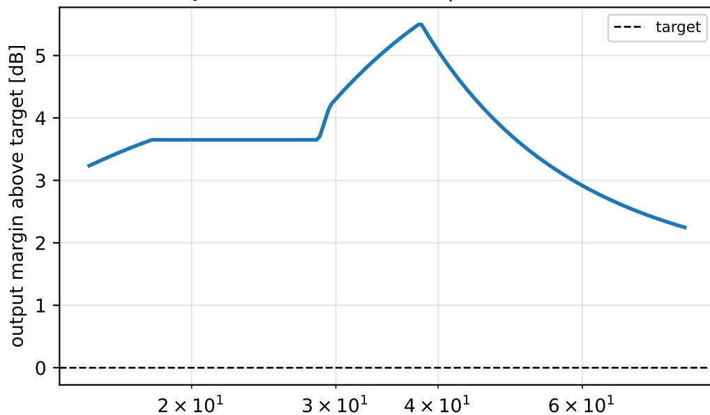
Dayton Audio UMII18-22 | sub manifold
