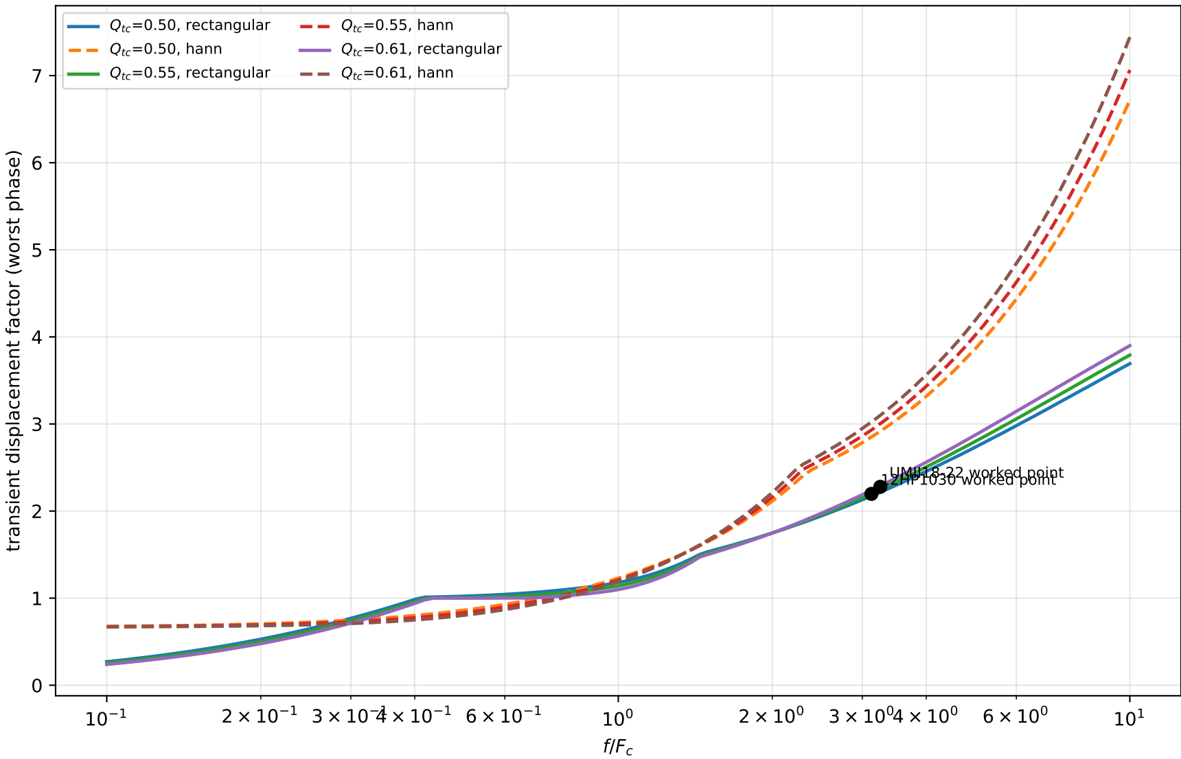
One-cycle burst transient factor vs. sealed-box alignment
