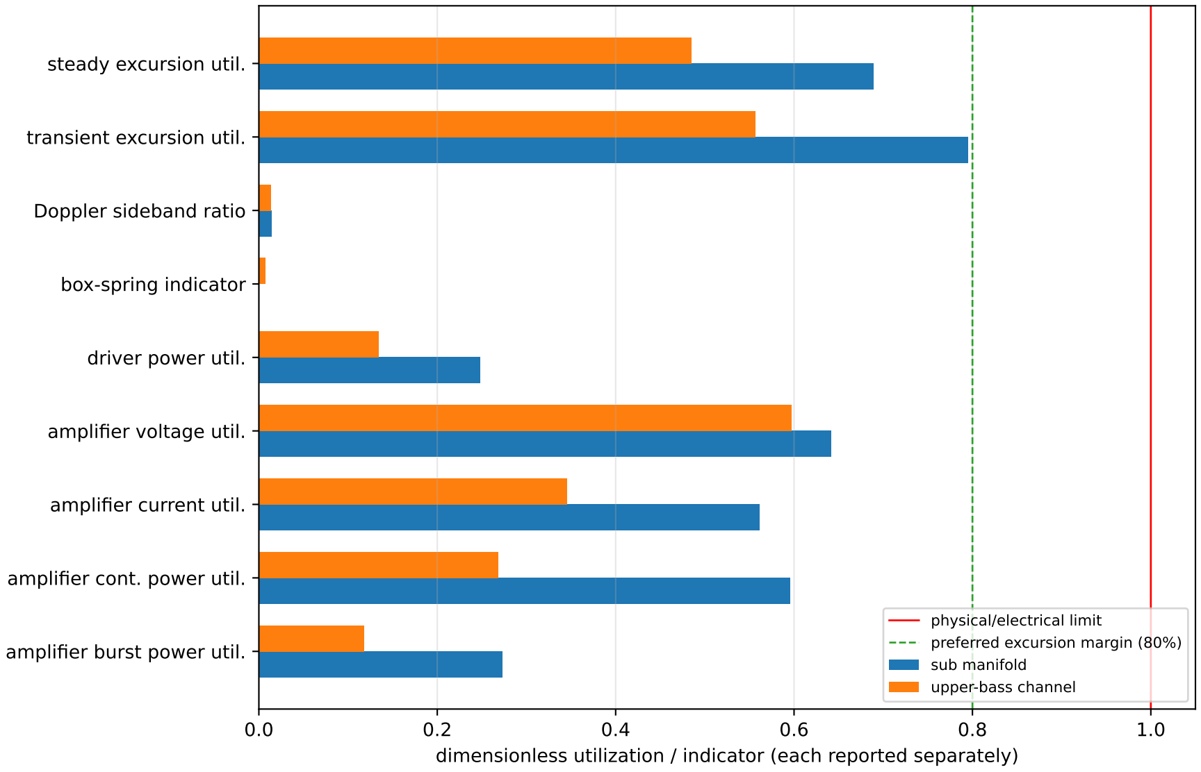
Dayton Audio UMII18-22 (sub) vs. FaitalPRO 12HP1030 (upper) — worked selected pair
