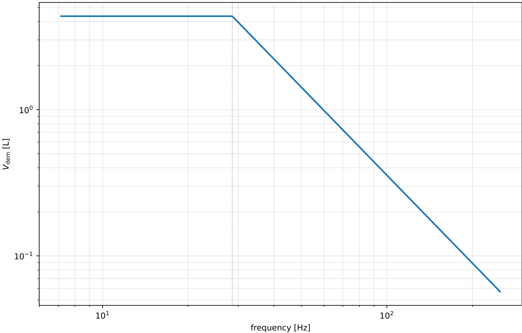
Required displaced volume at 110 dB, 3 m ( V_{\text{room}}=60 \text{ m}^3 , L_{\text{max}}=6 \text{ m} )
