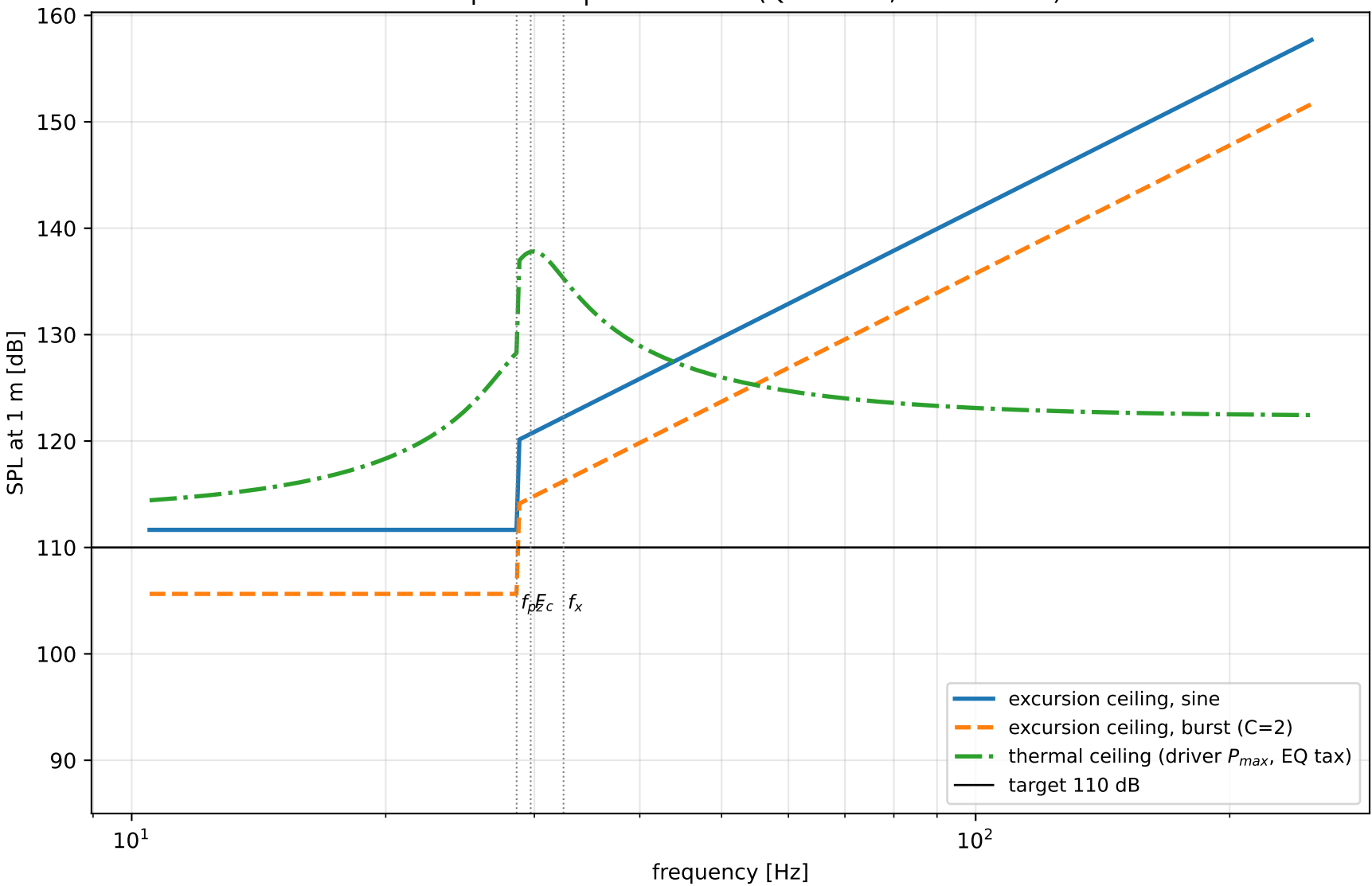
Example S18 | 2x in 246 L ( Q_{tc}=0.71 , F_c=29.7 Hz)
