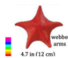
Bat star
