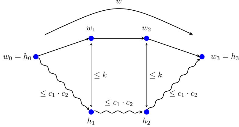
FIG. 4. L -quasi-convex subgroups are also L -proximate subsets of the group. Here w \in L \cap \pi^{-1}(H) , so by L -proximateness is in the k -neighbourhood of H , as shown by elements h_i . Then, for i \in [0, 2] , h_i^{-1}h_{i+1} \in H and |h_i^{-1}h_{i+1}|_S \leq 2k + 1 so |h_i^{-1}h_{i+1}|_T \leq c_1 , whence the path shown between h_i and h_{i+1} , which is labelled by elements of T^{\pm 1} , has S -length at most c_1 c_2 . AD: at least I hope this is what's shown.
