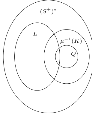
FIG. 1. L -representatives of a rational subset: L and Q are regular subsets of (S^\pm)^* and the projection \mu: L \rightarrow G makes (G, L) a rational structure. The subset K = \mu(Q) is rational in G , and its set of L -representatives is \mu^{-1}(K) \cap L which is not, in general, equal to Q \cap L .
