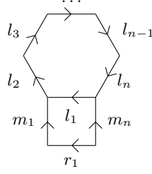
FIG. 30. Relations \tau = l_1 \dots l_n , \sigma = l_1 m_1^{-1} r_1^{-1} m_n as in P4 .
