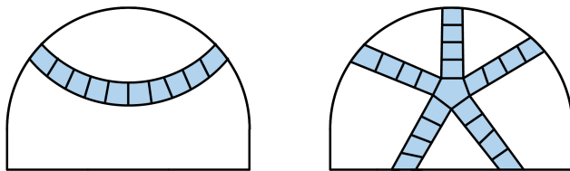
FIG. 2. Corridor (left) and spider (right).
