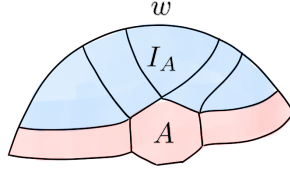
FIG. 17. Spider w -arc A in a disc diagram D , the majority of the spider's legs end in w . The region enclosed by A and \partial_w D is denoted I_A .
