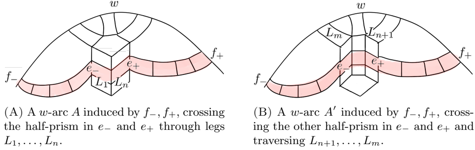
FIG. 19. On the left, a diagram D with a w -arc A traversing the lateral faces of a half-prism. A prismatic move yields the diagram D' on the right where A becomes A' and traverses the other lateral faces.
