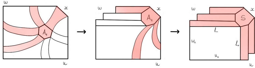
FIG. 26. C_x is a leg of an even-legged spider in Proposition 5.22.
