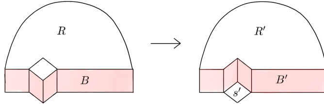
FIG. 12. Setup of Theorem 3.32
