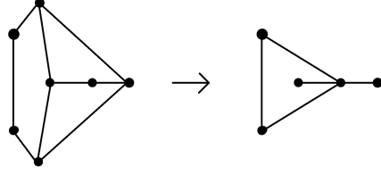
FIG. 16. Collapse of degenerate circular leg gives a not cyclically reduced head.
