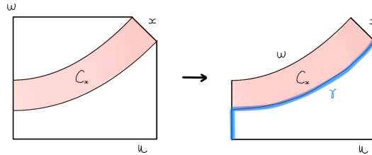
FIG. 24. C_x is not a leg of a spider in Proposition 5.22.
