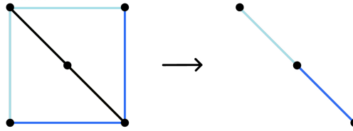
FIG. 7. Collapse of two squares.
