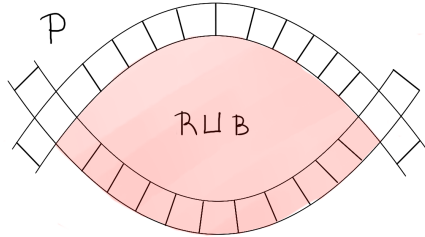
FIG. 14. Choosing the subcomplexes R and B in the double intersection from Theorem 3.32.
