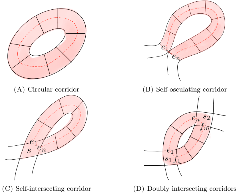
FIG. 9. In each image the dotted line shows a fibre and the shaded cells show the corresponding pathology P .
