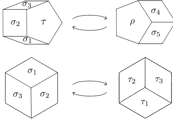
FIG. 6. Prismatic moves (above) and hexagonal moves (below).
