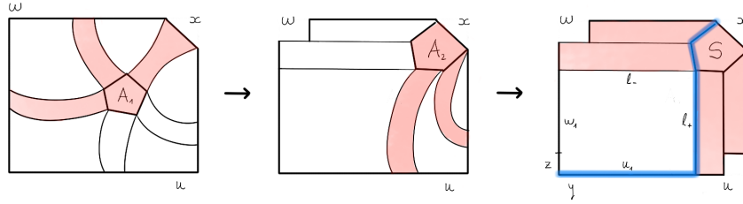
FIG. 25. C_x is a leg of an odd-legged spider in Proposition 5.22.
