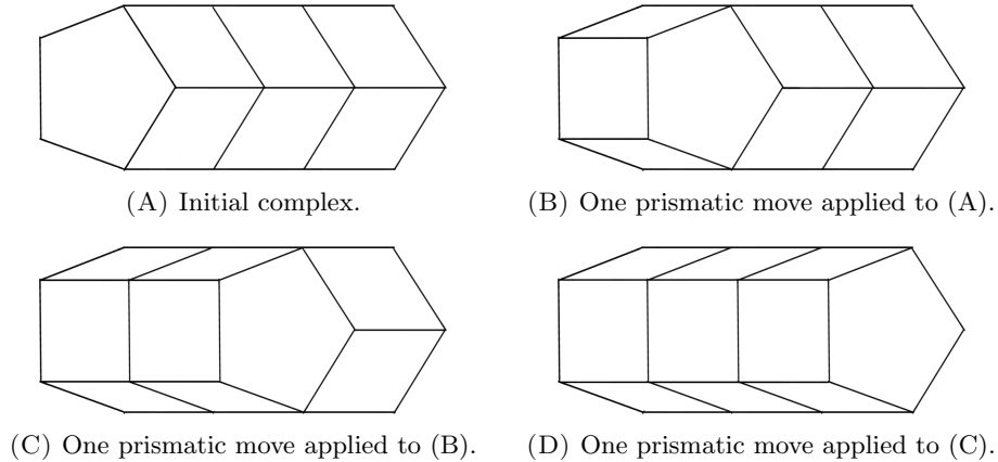
FIG. 8. Prismatic moves used sequentially to deal with longer prisms, where first and last complex are understood as prisms of height three.
