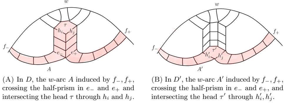
FIG. 18. On the left, a diagram D with a w -arc A traversing the base of a half-prism. A prismatic move yields the diagram D' on the right where A becomes A' and traverses the other base.
