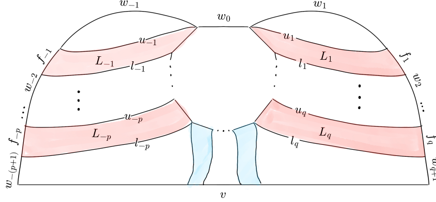
FIG. 20. Spider w -arc in a disc diagram D for a word wv^{-1} where the spider's head intersects \partial_w D : each leg L_i in the w -arc as an upper side u_i and a lower side l_i , the end edges of the legs break the path w into a concatenation of f_i -edges and w_i -paths, and the region enclosed by w_i , u_i and l_{i-1} is denoted by R_i .
