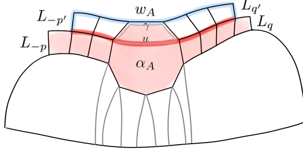
FIG. 22. Inner shortcut for an empty spider w -arc A determined by the legs L_{-p} and L_q . The portion of the head \gamma lying between L_{-p'} and L_{q'} has a non-geodesic label, that can be shortened to u .
