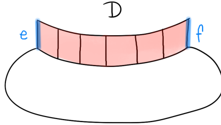
FIG. 11. Diagram with an arc at its boundary.
