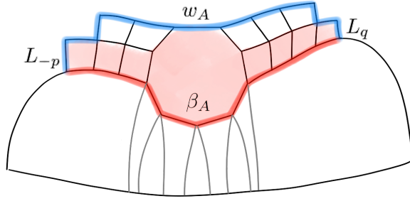
FIG. 23. Outer shortcut for an empty spider w -arc A .
