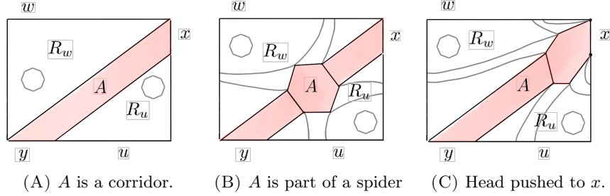
FIG. 27. Definition of the subcomplex A and the regions R_w, R_u (which may contain spider heads) depending on whether the edge y defines a corridor or a spider. If A belongs to a spider, its head can be pushed against the edge x .
