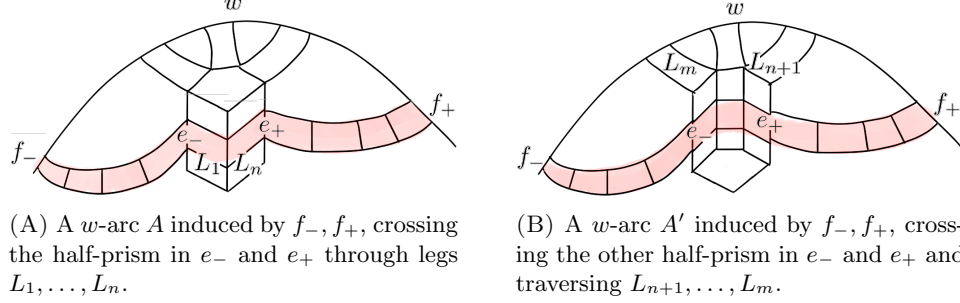
FIG. 20. On the left, a diagram D with a w -arc A traversing the lateral faces of a half-prism. A prismatic move yields the diagram D' on the right where A becomes A' and traverses the other lateral faces.
