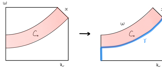
FIG. 24. C_x is not a leg of a spider in Proposition 6.2.
