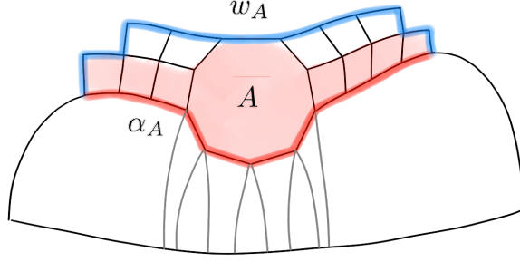
FIG. 23. Shortcut for an empty spider w -arc A .
