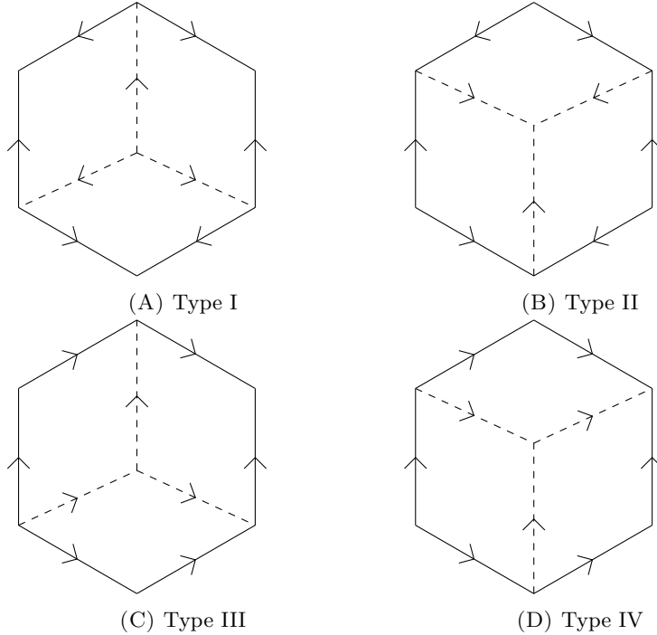
FIG. 33. Four types of half-cubes over trickle groups.
