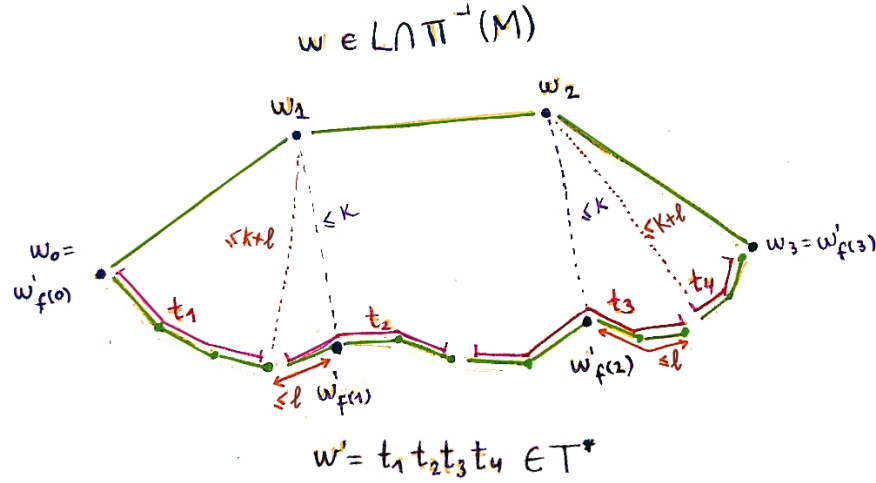
FIG. 3. Weakly- L -proximate submonoids are L -proximate. The distance in w' between w'_{f(1)} and w'_{f(2)} is bounded by the distance in w' between the initial vertex of t_2 \in T and the final vertex of t_3 \in T . These vertices sit at most l edges along w' away from w'_{f(1)} and w'_{f(2)} respectively, so their distance in S -metric is bounded by 2(k + l) + 1 .
