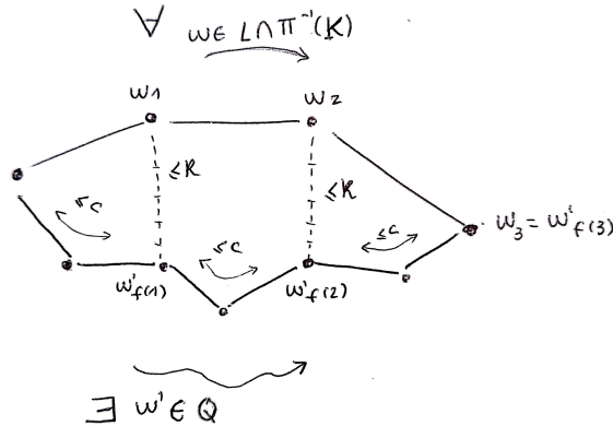
FIG. 2. Illustration of the paths in the Cayley graph defined by the words \bar{w} , w' in Definition 3.1.
