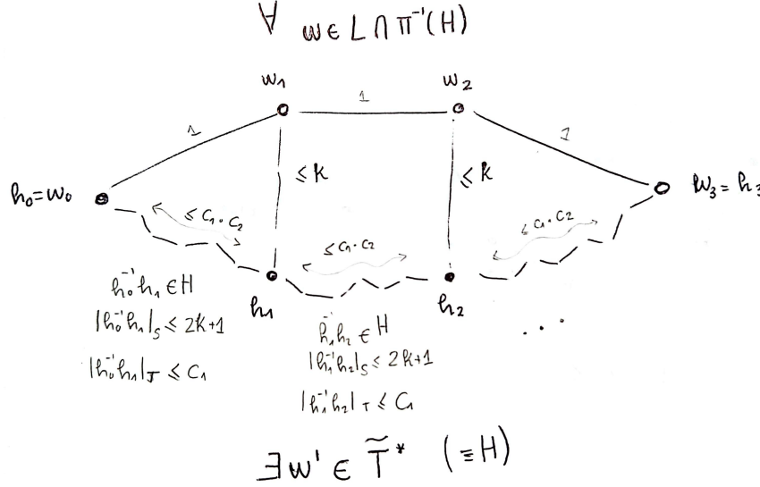
FIG. 4. L -quasi-convex subgroups are also L -proximate subsets of the group.
