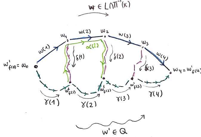
FIG. 5. Notation for the proof of Proposition 4.9
