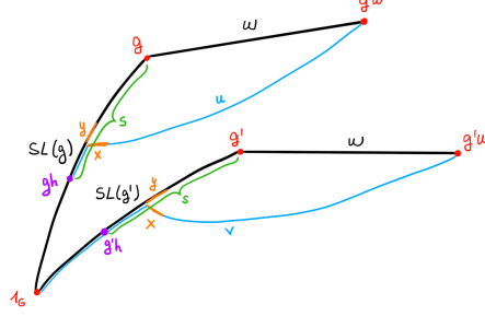
FIG. 25. Case 2.2.A in the proof of Lemma 6.6.
