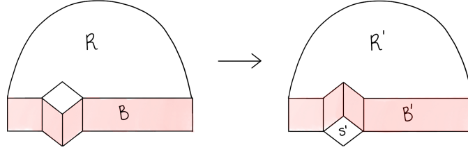
FIG. 13. Setup of Theorem 4.20
