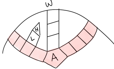
(A) A w -arc containing a spider head H .
