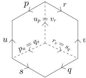
FIG. 42. Labelling for a half-cube of type I.
