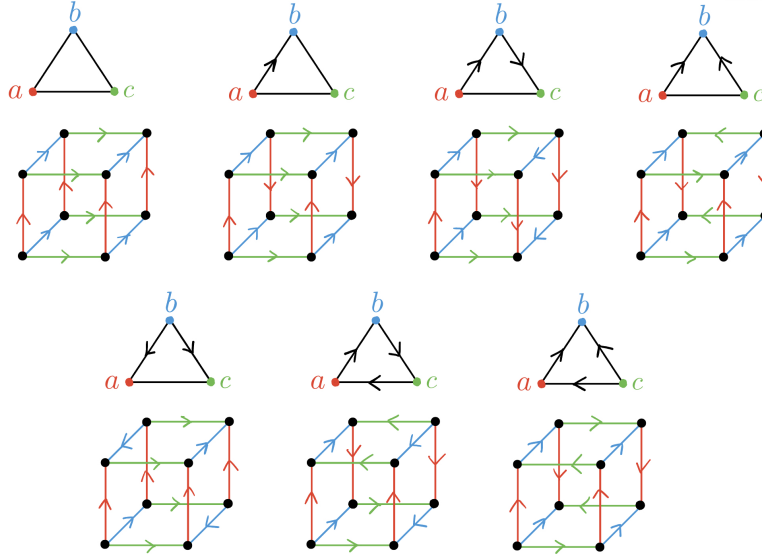
FIG. 43. Cubes in the Cayley complex of a T-RAAG.
