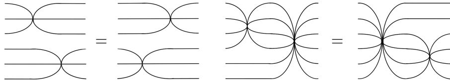
(B) Commuting generators.
