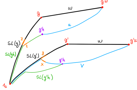
FIG. 27. Case 2.2.C in the proof of Lemma 6.6.
