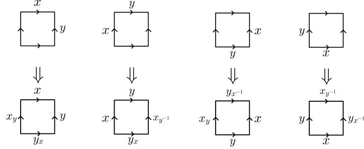
FIG. 33. Any two consecutive edges determine the rest.
