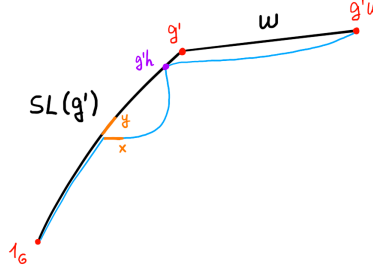
FIG. 26. Case 2.2.B in the proof of Lemma 6.6.
