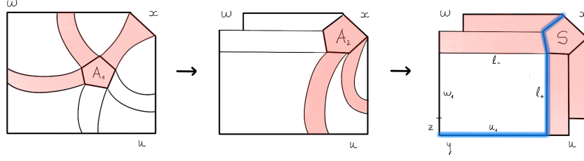
FIG. 29. C_x is a leg of an odd-legged spider in Proposition 7.2.
