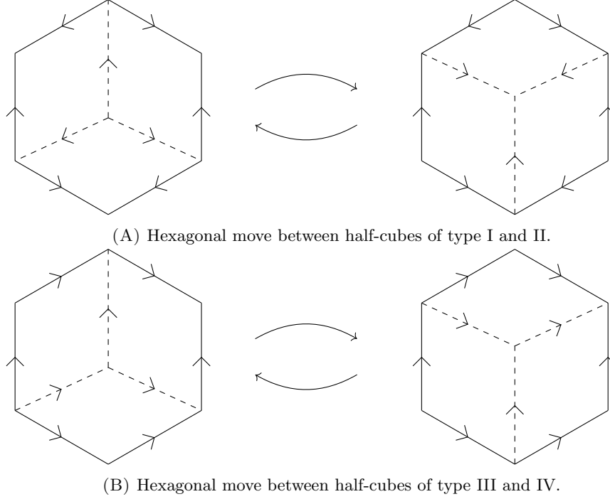
FIG. 39. The four types of half-cubes come in complementary pairs.
