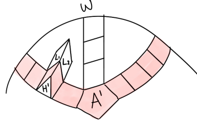
(B) H can be pushed out to H' using a prismatic move.
