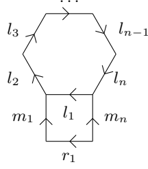
FIG. 34. Relations \tau = l_1 \dots l_n , \sigma = l_1 m_1^{-1} r_1^{-1} m_n as in P4 .
