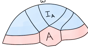
FIG. 18. Spider w -arc A in a disc diagram D , the majority of the spider's legs end in w . The region enclosed by A and \partial_w D is denoted I_A .
