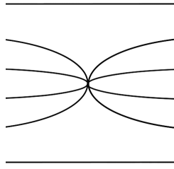
FIG. 4. A generator in a cactus group corresponding to an interval of size 4.
