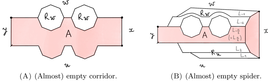
FIG. 32. Once the (yux^{-1}) -arc and the (y^{-1}wx) -arc defined by A are emptied, all the heads from R_u \cup R_w are pushed against R_w and they all intersect A , so w and u K -fellow travel.
