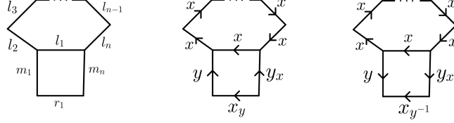
FIG. 37. \tau and \sigma in a trickle group
