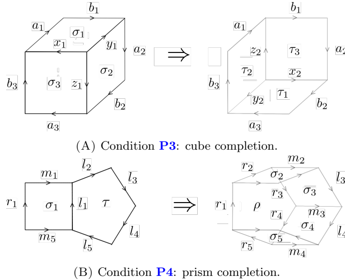
FIG. 7. Conditions for prismatic presentation following notation in Definition 3.6, see Fig. 1 for an unlabelled version.
