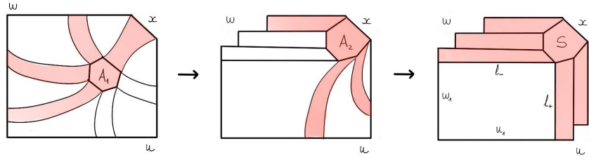
FIG. 30. C_x is a leg of an even-legged spider in Proposition 7.2.
