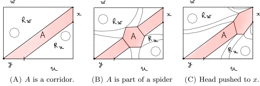
FIG. 31. Definition of the subcomplex A and the regions R_w, R_u (which may contain spider heads) depending on whether the edge y defines a corridor or a spider. If A belongs to a spider, its head can be pushed against the edge x .
