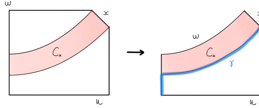
FIG. 28. C_x is not a leg of a spider in Proposition 7.2.
