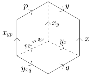
FIG. 41. Labelling for a type III hexagon.
