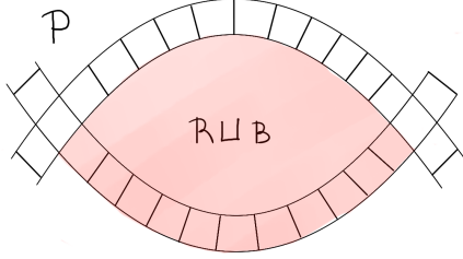
FIG. 15. Choosing the subcomplexes R and B in the double intersection from Theorem 4.20.
