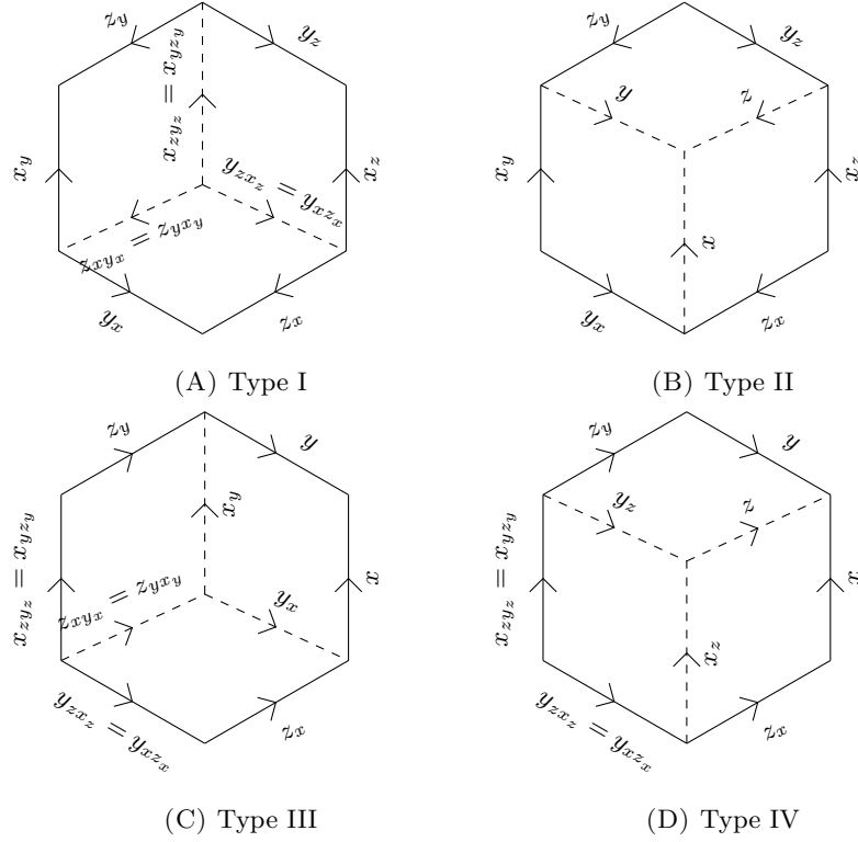
FIG. 40. Tessellated hexagons can always be labelled like this for some generators x, y, z .
