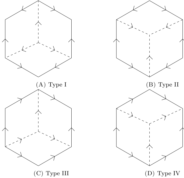
FIG. 38. Four types of half-cubes over trickle groups.
