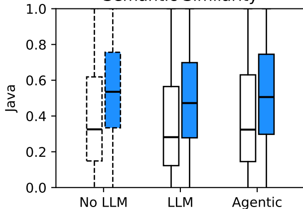
Semantic Similarity
