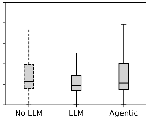
Syntactic Similarity
