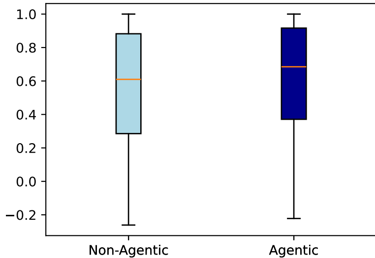
Cosine Similarity
