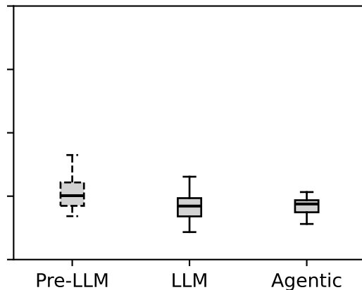
Syntactic Similarity
