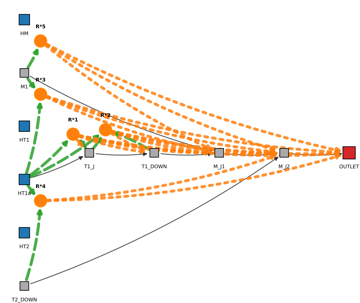
Physicalised (5 reservoirs, backflow share=0.21)
