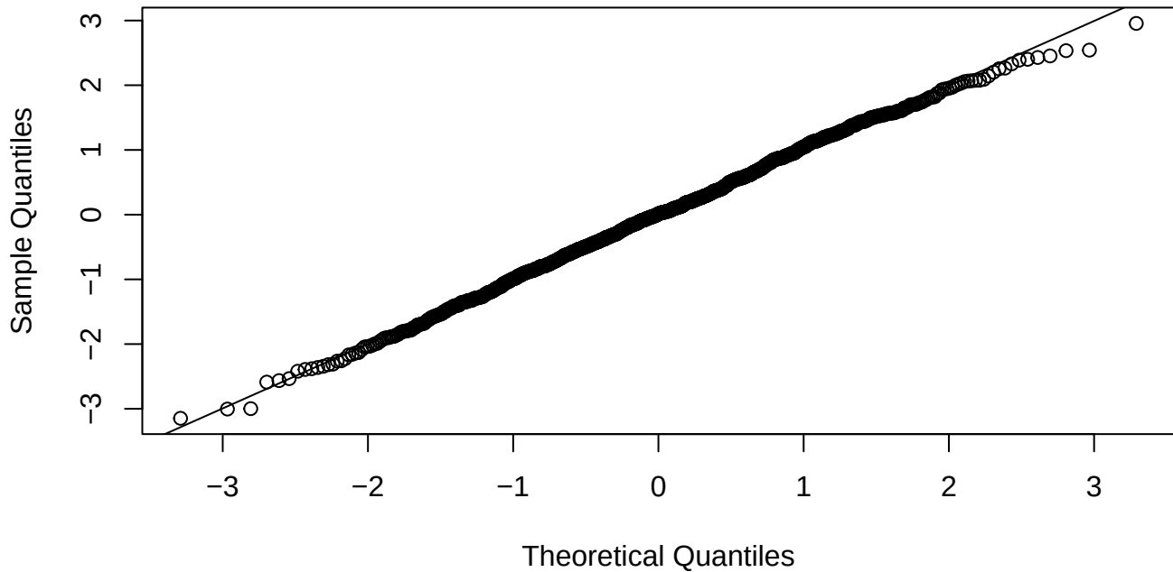
Column 8
