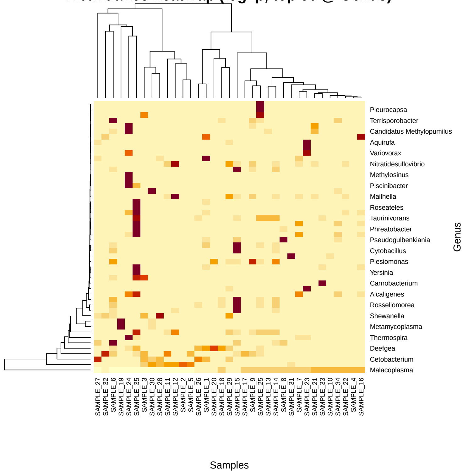
Abundance heatmap (log1p, top 50 @ Genus)
