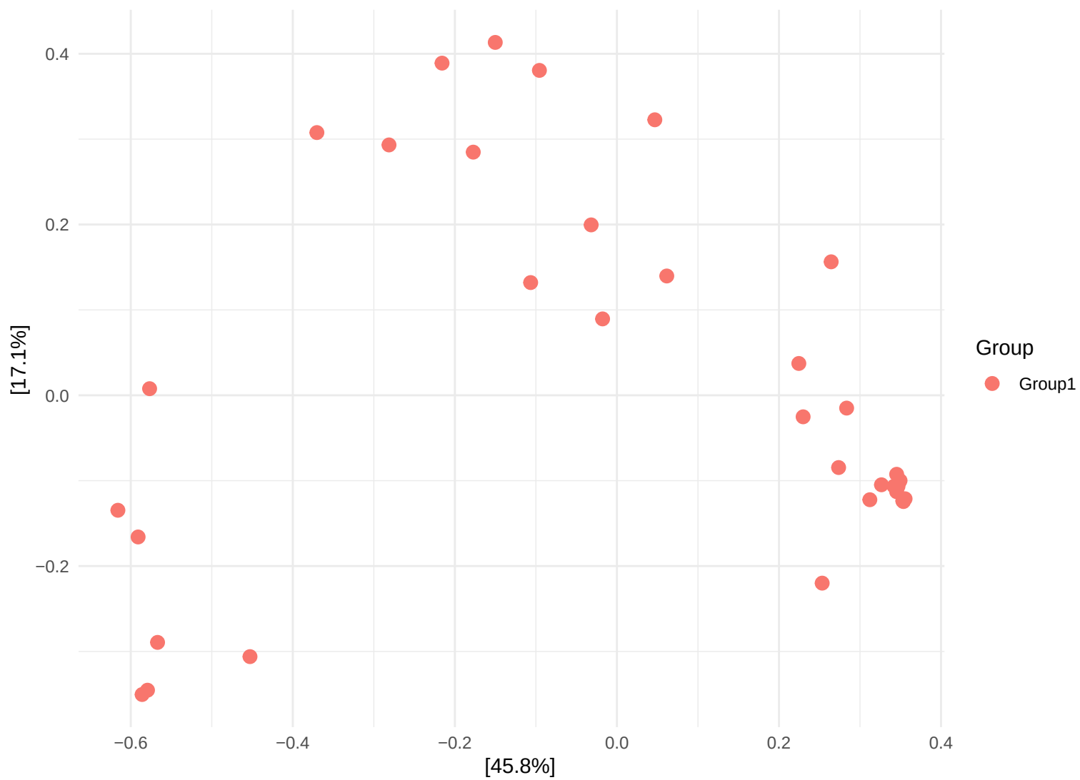
PCoA (Bray–Curtis)
