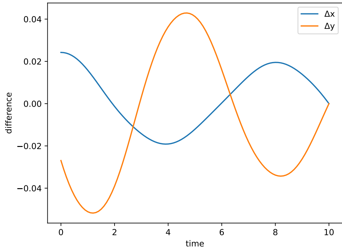
Forward vs Backward Difference
