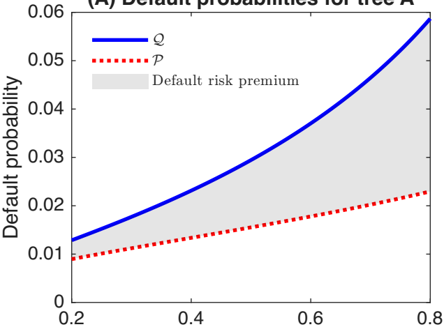
(A) Default probabilities for tree A
