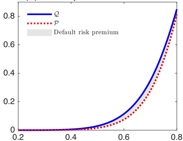
(B) Default probabilities for tree B
