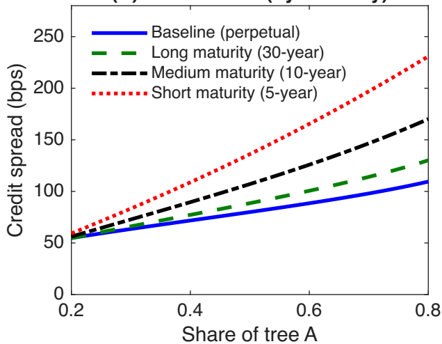
(C) CS of tree A (by maturity)
