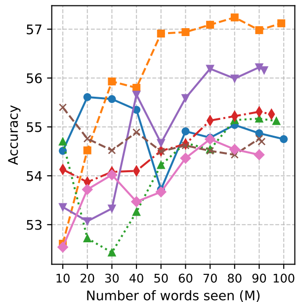
BLIMP
