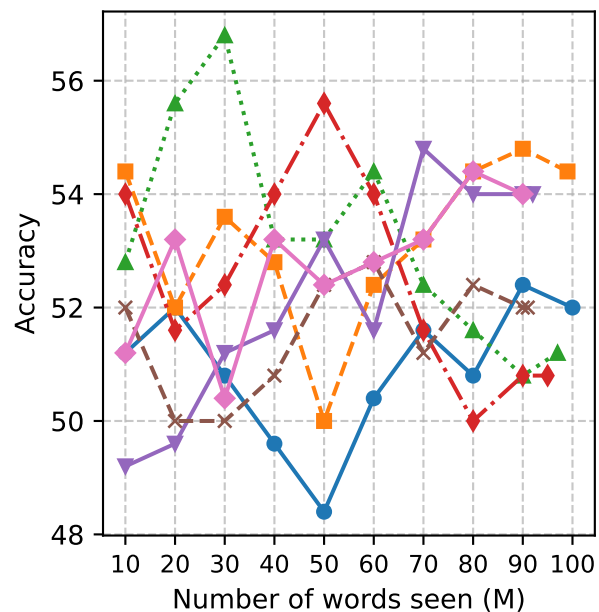
SUPPLEMENT
