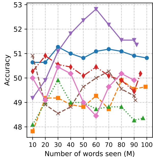
EWOK
