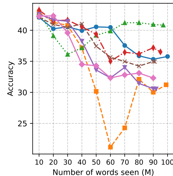
ENTITY TRACKING
