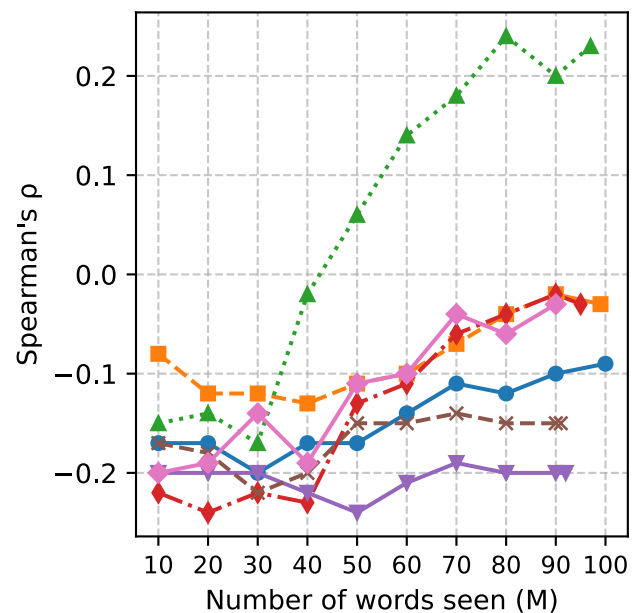
WUG PAST
