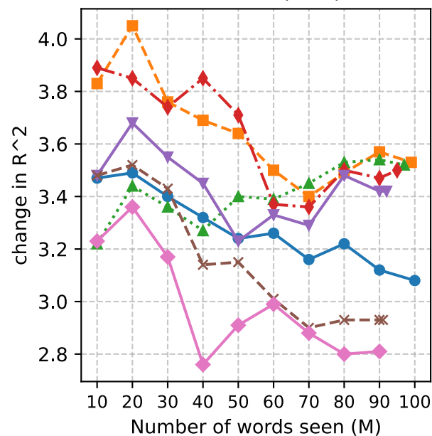
READING (SPR)
